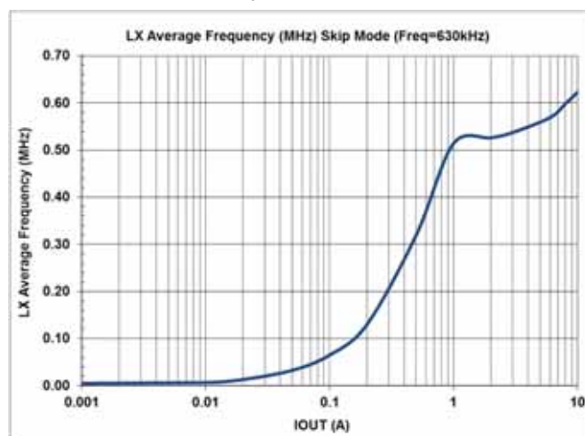
Frequency = 630 kHz
