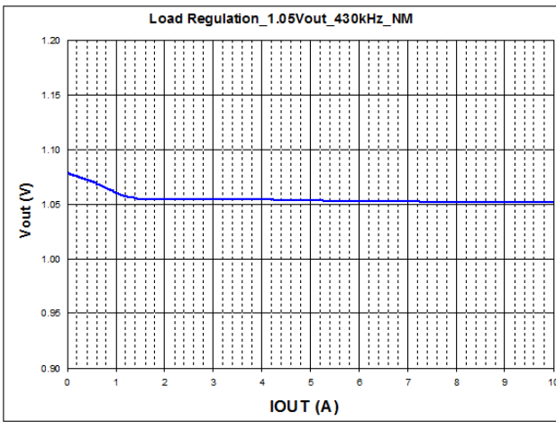
Frequency = 430 kHz
