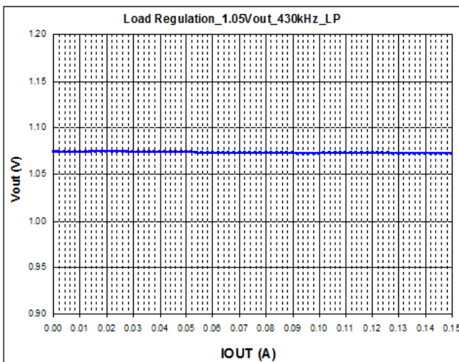
Frequency = 430 kHz
